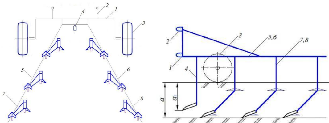
1-frame; 2-hanging device; 3-base wheels; 4-softening paw; 5 and 6 – frame of left and right sections; 7-softeners with slanted columns bent to the right; 8-bent to the left inclined pillar softeners;
