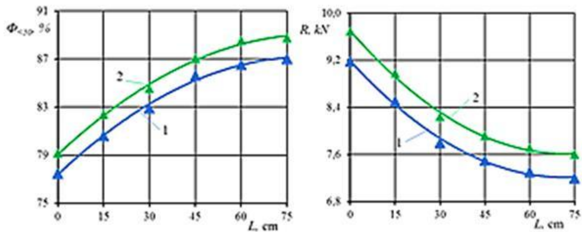
Figure 3. The level of soil compaction ( \Phi_{<50} ) and the traction resistance ( R ) of the inclined column working bodies depending on the longitudinal distance ( L ) between them o'zgarishi
